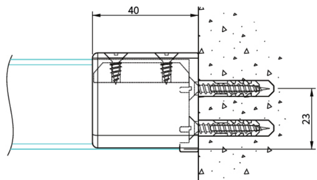
Wall fixing with bracket
