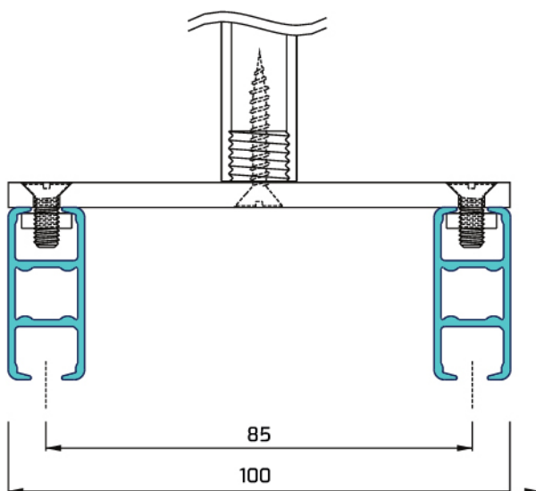
Parallel rail fixing with bridging plate
